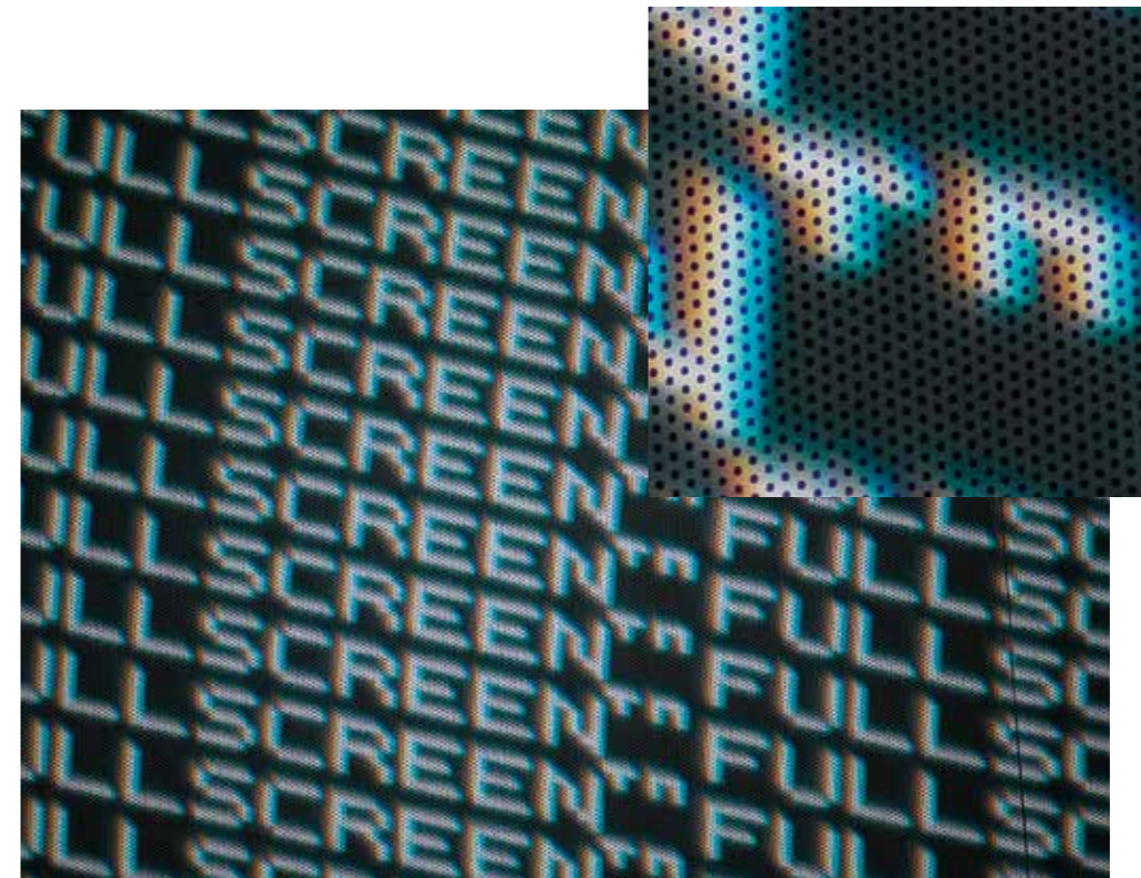
Segment of projected image, F35/NAVITAR HM117/11.7 – (test image) Lateral color: clearly visible – 2 to 3 pixel widths Exposure data: Canon EOS 5D Mk II, ZEISS Macro-Planar 2/100
