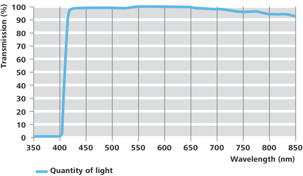
ZEISS T* UV filter
