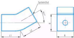
Angle piece, M5 626105-6020-050
