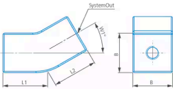
Angle piece, M5 626105-6020-015
