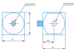
Cube, M5 Titanium 20 mm with removeable screw 626115-6110-003
