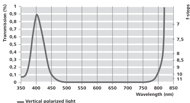
ZEISS T* POL filter (circular)
