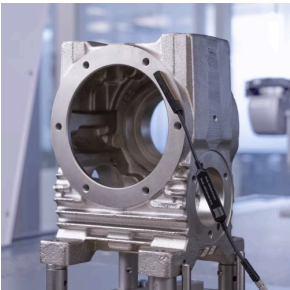
Temperature sensor (mini) magnetic, M5
