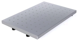
THETA 32 pallet, M6 25x25 grid, Aluminum 626109-9220-021
