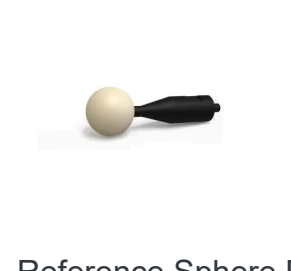
Reference Sphere DK 25, DG 18, M6 (μ50 porosity)
